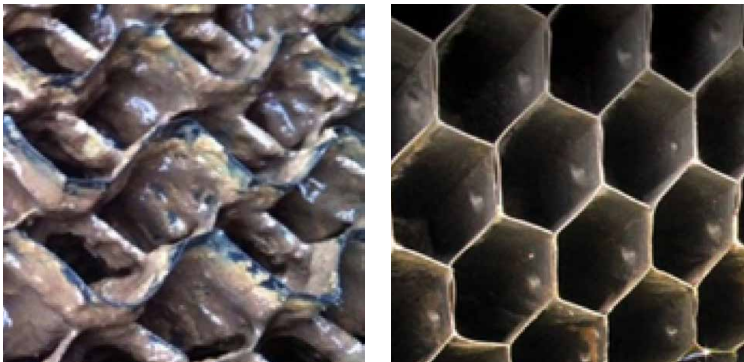
Cooling tower lamellas, before and after switching to HeiQ Synbio Aquatec treatment
